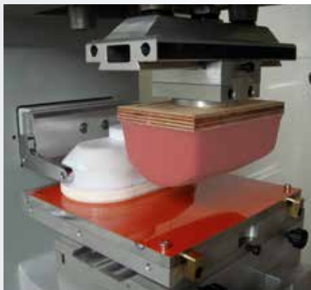
Ink-cup cross-table
